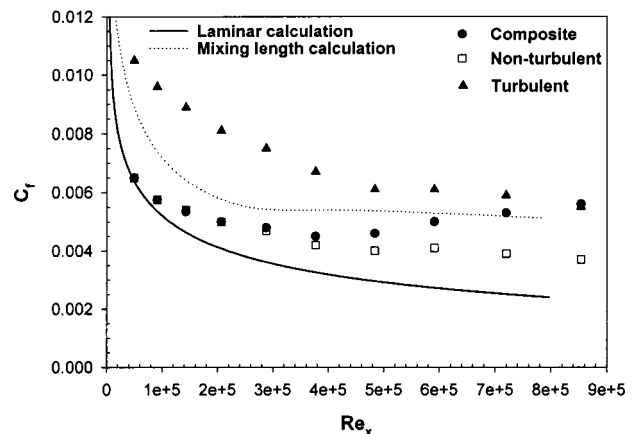
Fig. 10 Skin-friction coefficient
