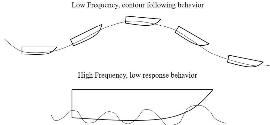
Figure 4.17: Relationship between wave length and ship response
