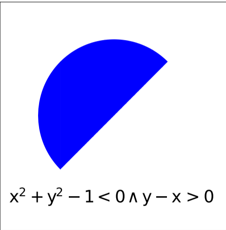
Semi-Algebraic Set
