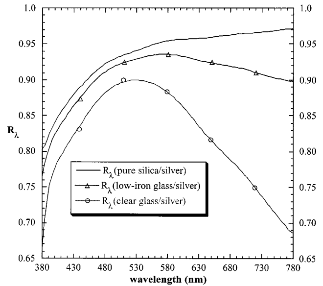
Fig. 10. Simulated spectral reflectances R_\lambda for several types of second-surface glass mirrors, modeled using Eqs. (2)–(5). Each simulation assumes normal incidence and includes external specular reflections from the mirror glass, multiple reflections from within the mirror, and a 5 mm thick glass substrate.
