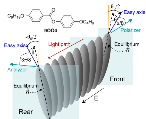
FIG. 1 (color online). Schematic diagram of experimental geometry for a right-handed twist cell. \theta_0 is the rotation angle between the front and rear easy axes and \theta is the deviation of the equilibrium director orientation \hat{n} (dashed line) from the easy axis at the front substrate. Note that \theta is negative for a right-handed twist. The electric field \vec{E} is shown, and the laser light path runs from the front to the rear substrate. Analyzer is rotated counterclockwise from polarizer by an angle -(\pi/2 + \theta_0) . Inset: Chemical formula for 9004.
