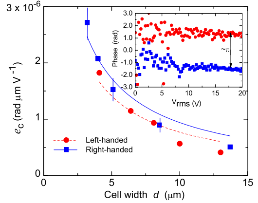
FIG. 3 (color online). Electroclinic coefficient e_c at \omega = 2\pi \times 1000 \text{ Hz} versus cell width d . Red circles and dashed fit are for the left-handed cell and blue squares and solid fit for the right-handed cell. Error bars for e_c are shown; uncertainty in d is approximately the size of the symbols. Each cell may have a small systematic error due to the uncertainty in \theta_0 . Inset: Relative phase of ac signal for left- and right-handed cells at d \sim 8.1 \pm 0.2 and 8.5 \pm 0.2 \mu\text{m} , respectively, showing a phase difference of approximately \pi .
