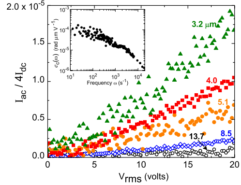
FIG. 2 (color online). The intensity ratio I_{ac}/4I_{dc} versus applied voltage for five different cell widths d in the right-handed cell: Solid green triangles, 3.2 \mu\text{m} ; solid red squares, 4.0 \mu\text{m} ; solid orange circles, 5.1 \mu\text{m} ; open blue diamonds, 8.5 \mu\text{m} ; open black circles, 13.7 \mu\text{m} . The uncertainty in d is \pm 0.2 \mu\text{m} . Inset: Electroclinic coefficient e_c(\omega) versus frequency at fixed voltage of 8 V_{\text{rms}} and d = 3.2 \mu\text{m} .
